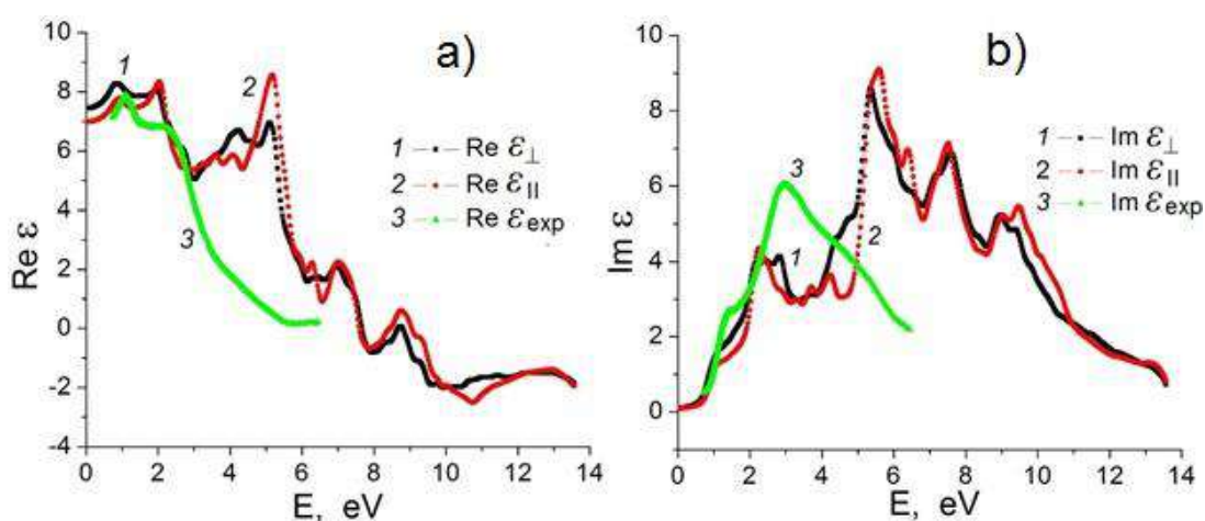
Fig. 1. Real ( \text{Re } \epsilon ) (a) and imaginary ( \text{Im } \epsilon ) (b) parts of the dielectric function of CuInS 2 (1, 2 - theory; 1 - perpendicular to the tetragonal axis c ( \perp ), 2 - along the tetragonal axis c ( \parallel ), 3 - experiment).
